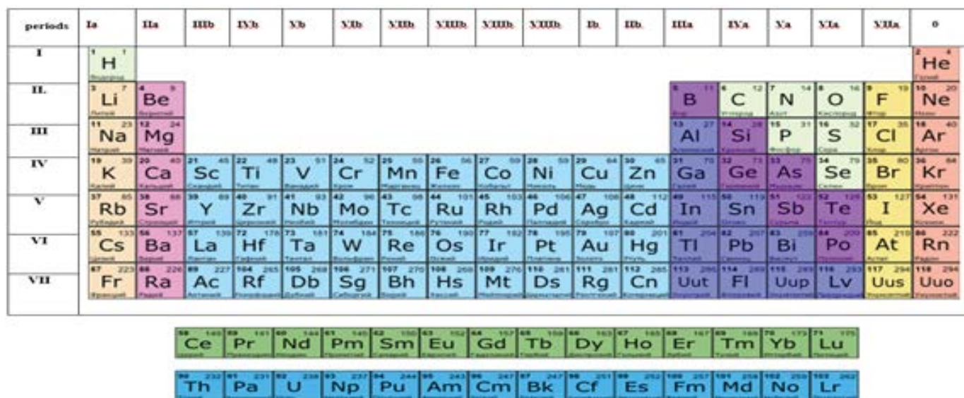
Figure 1: Long version of the traditional Mendeleev's table.
