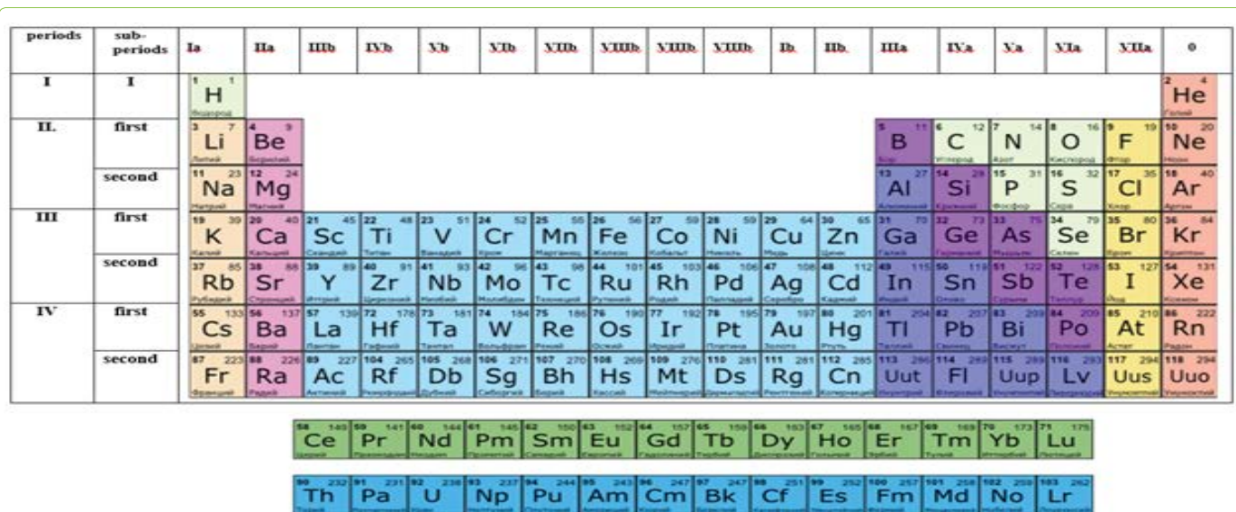
Figure 2: Reconfigured long version of the Mendeleev's table.
