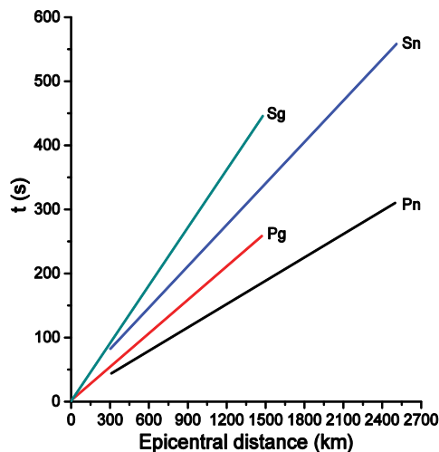
(a) (b) Figure 26: Mohorovičić travel-time curve (a) (Courtesy of the Department of Geophysics, Faculty of Science, Zagreb) [166] and (b) best fitting curves.
